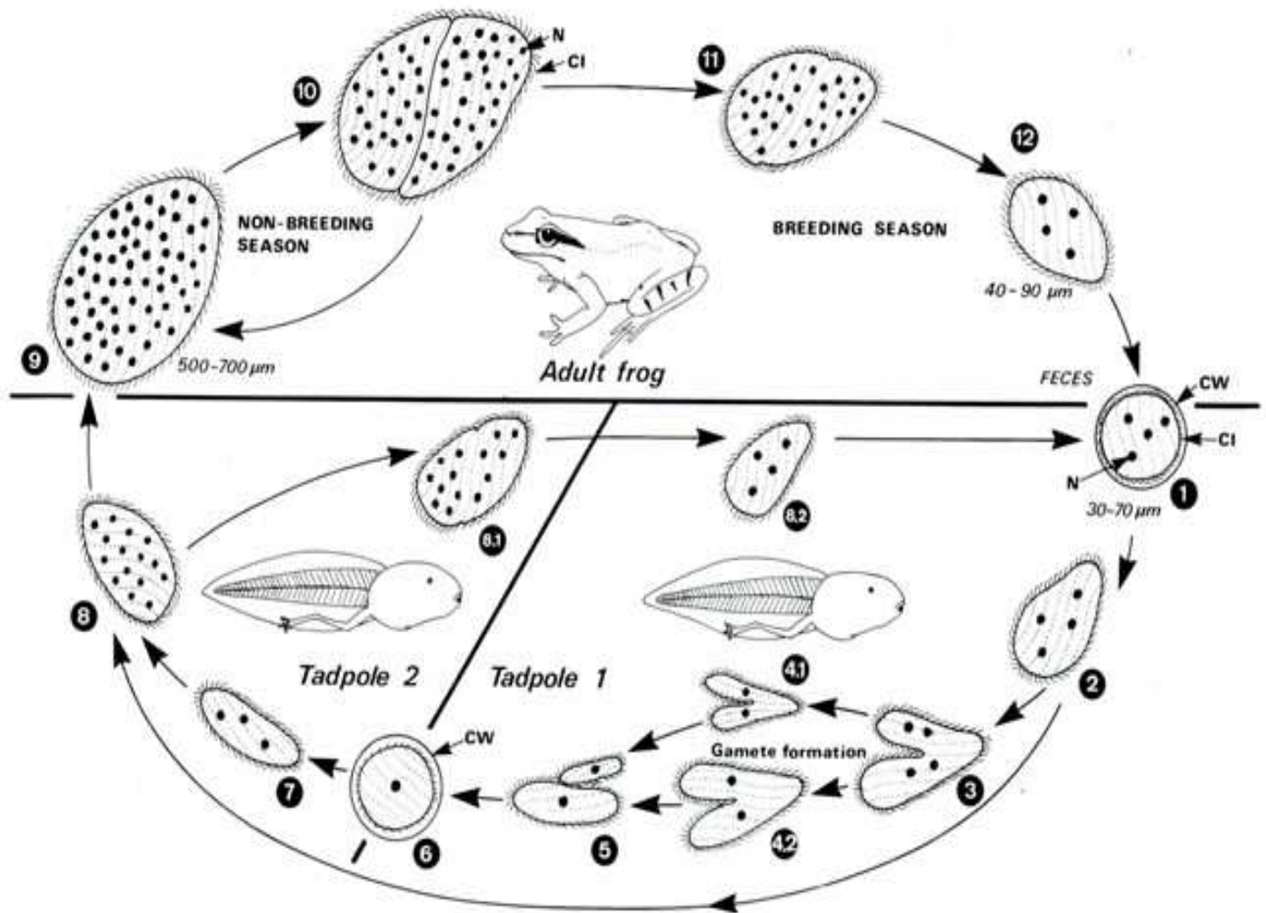
Fig. 1.8. Life cycle of Opalina ranarum . 1 Cysts are excreted by the adult frog and orally ingested by a tadpole. 2 After hatching the young gamont migrates to the cloaca. 3, 4 Formation of micro- and macrogametes (meiosis). 5 Fusion of the heterogametes. 6 Encystation of the zygote and excretion via feces. 7, 8 After oral uptake of a cyst by another tadpole the trophozoite grows up in the cloaca (up to 0.5 mm). 8.1, 8.2 The small trophozoite may start division inside the tadpole, finally leading to formation and excretion of cysts (1) which give rise to new trophozoites (2→8) after ingestion by another tadpole. 9 When metamorphosis of tadpoles to
